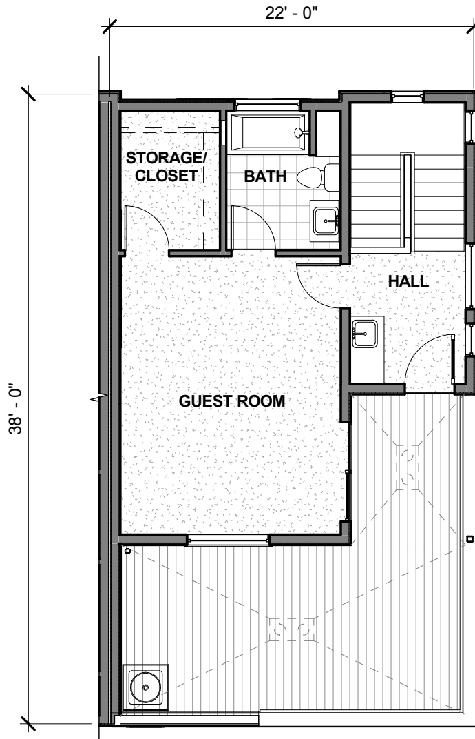
FOURTH FLOOR PLAN (UNIT 1)
