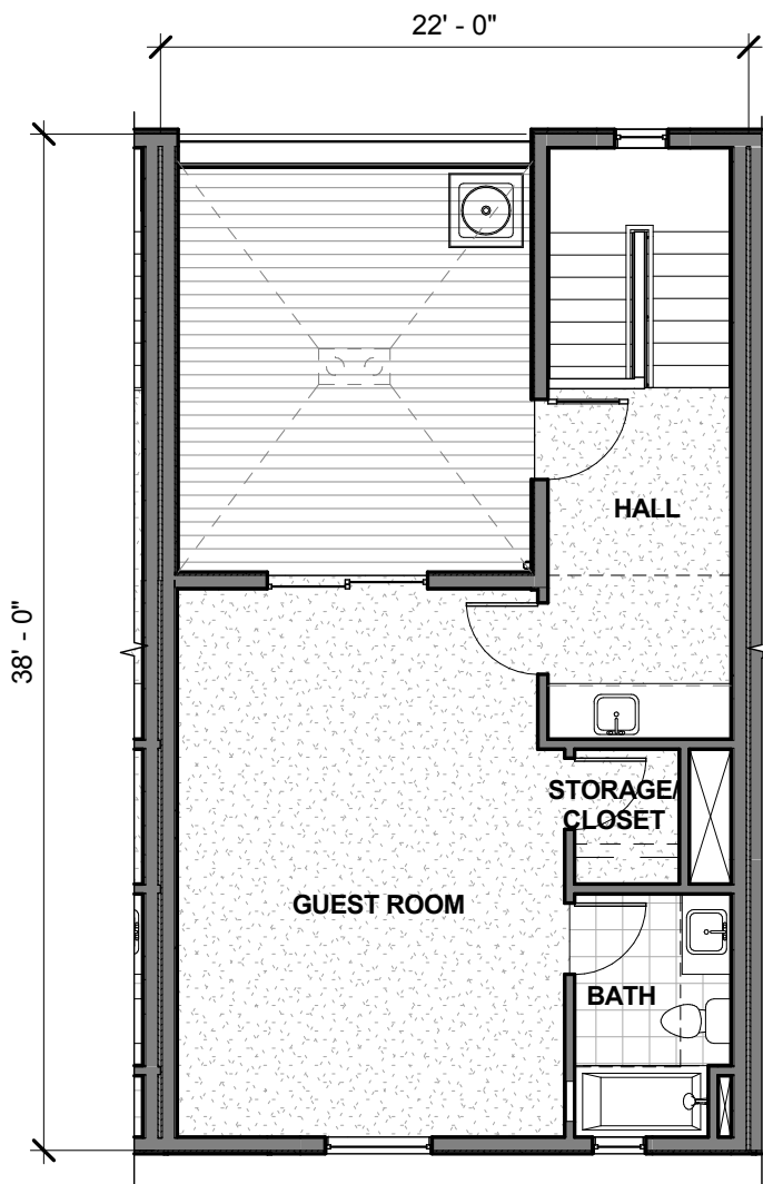
FOURTH FLOOR PLAN (UNIT 2-5)
