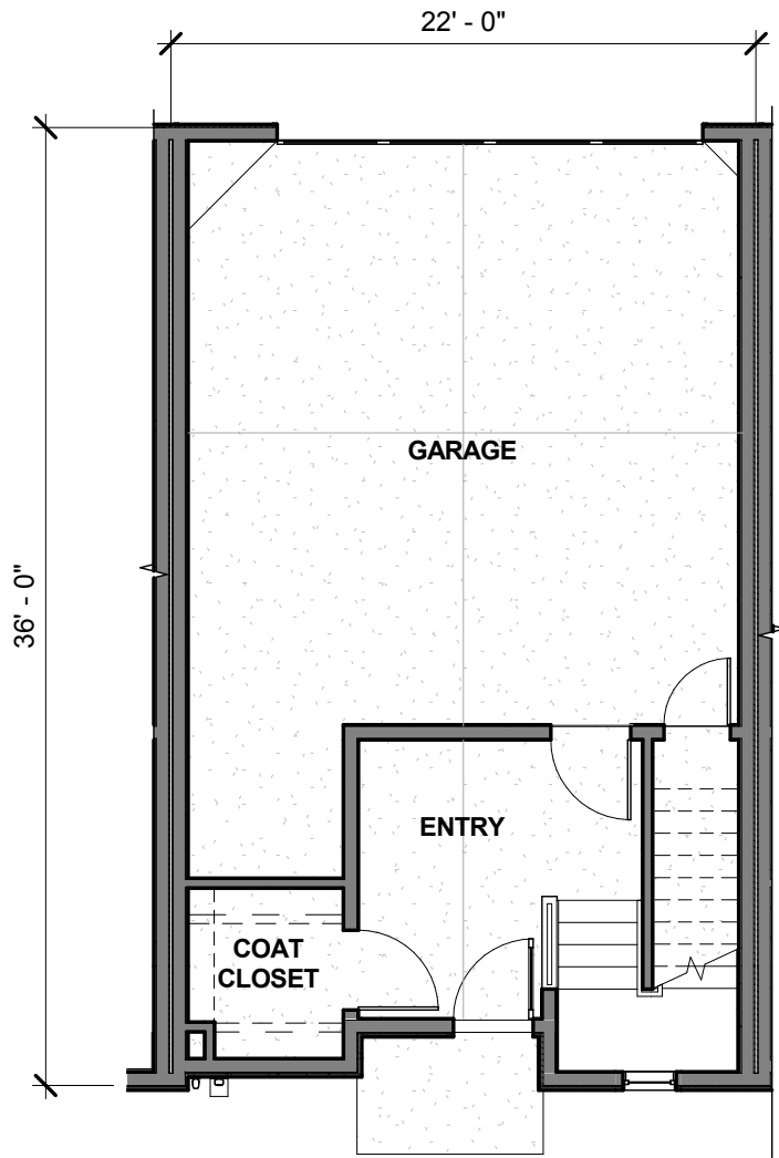
FIRST FLOOR PLAN (UNIT 2-5)
