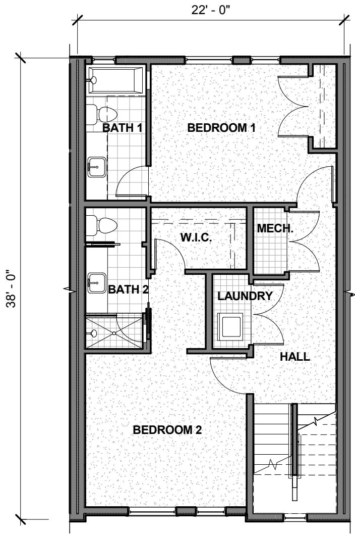
THIRD FLOOR PLAN (UNIT 2-5)
