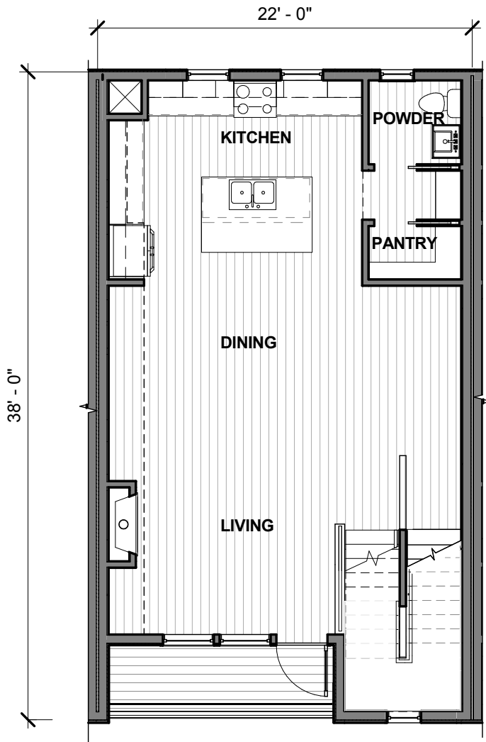
SECOND FLOOR PLAN (UNIT 2-5)
