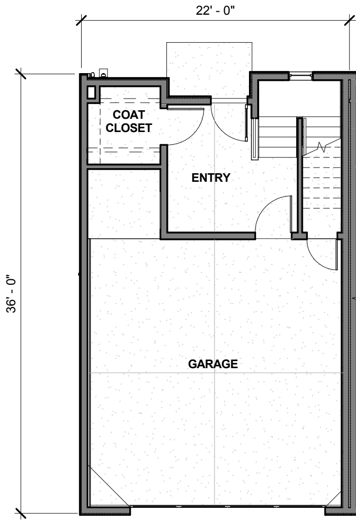
FIRST FLOOR PLAN (UNIT 6)
