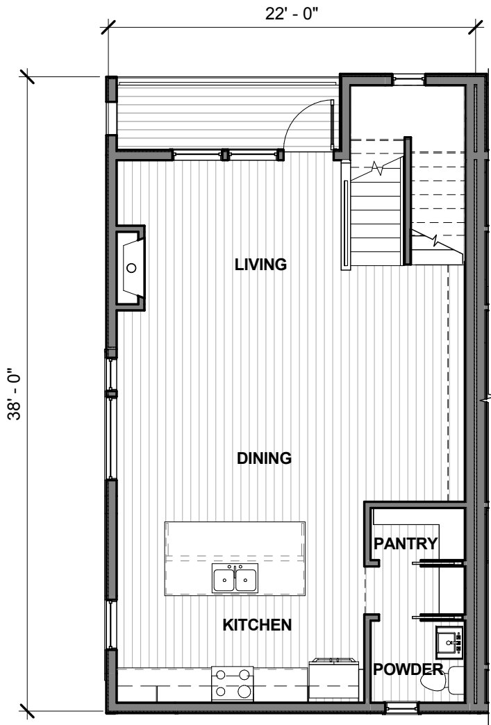
SECOND FLOOR PLAN (UNIT 6)
