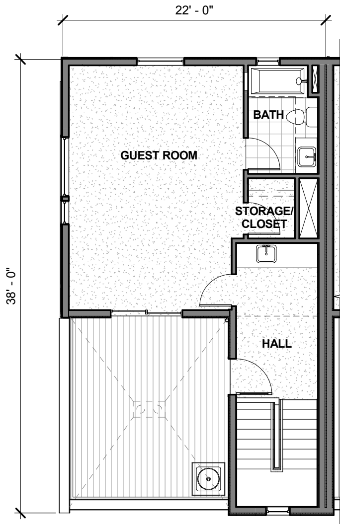
FOURTH FLOOR PLAN (UNIT 6)
