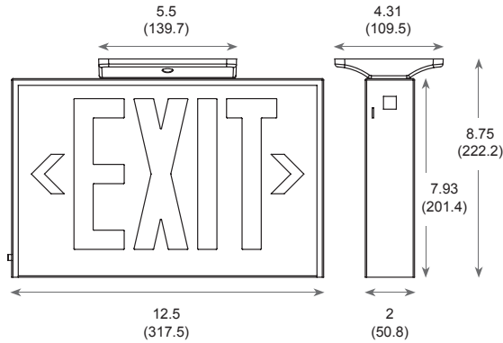
All dimensions are in inches (millimeters).
