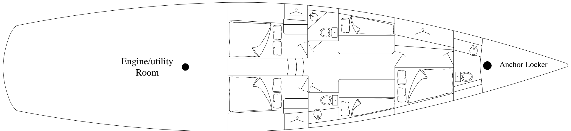
Below deck
