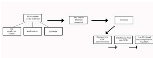
Figure 2. System architecture for SALTO.
