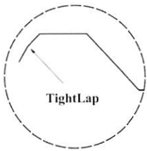
PBR Panel w/ TightLap Used for roof and wall applications. Minimum Slope is 1/2:12.
