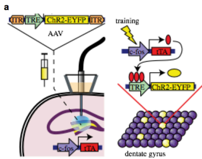
Figure 1: Engineering active hippocampus cells to express ChR2. Mice are injected with c-fos-tTA and TRE-ChR2 into the hippocampus, followed by optic fiber implants. When Dox is not present in an animal's diet, memory formation activates the c-fos promoter which subsequently drives the expression of the transcription factor tTA. Next, tTA binds to the promoter TRE which drives the expression of ChR2, thereby labeling a population of active cells (yellow).
