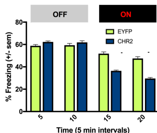
Figure 3: Activated positive memories suppress fear. Subjects were fear conditioned and then given a fear recall test. Comparable levels of freezing are observed in the first 10 minutes (OFF) between control EYFP and experimental ChR2 groups; when a positive memory is reactivated (ON) in the last 10 minutes, the ChR2 group shows attenuated freezing.
