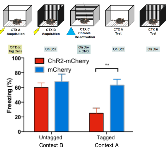
Figure 4: Subjects were first fear conditioned in context A and active HPC cells were tagged with ChR2. Next, these subjects were fear conditioned in context B but without further tagging of any HPC cells. In context C, cells that were originally active and tagged in context A were chronically stimulated. When placed back in context A, the experimental ChR2-mCherry group displayed robust decreases in freezing relative to mCherry controls; moreover, the effect was context-specific and did not elicit any changes in fear behavior when placed back in untagged context B.
