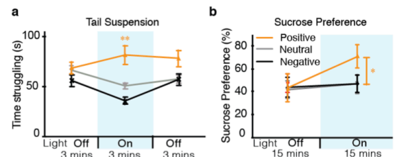
Figure 2: Activating a positive engrams rescues depression-like behavior. (A-B) Optical reactivation of dentate gyrus cells that were previously active during positive (orange), but not neutral (gray) or negative (black) memory formation significantly increases time struggling in the tail suspension test (a) and preference for sucrose (b). (Modified from Ramirez et al. 2015)
