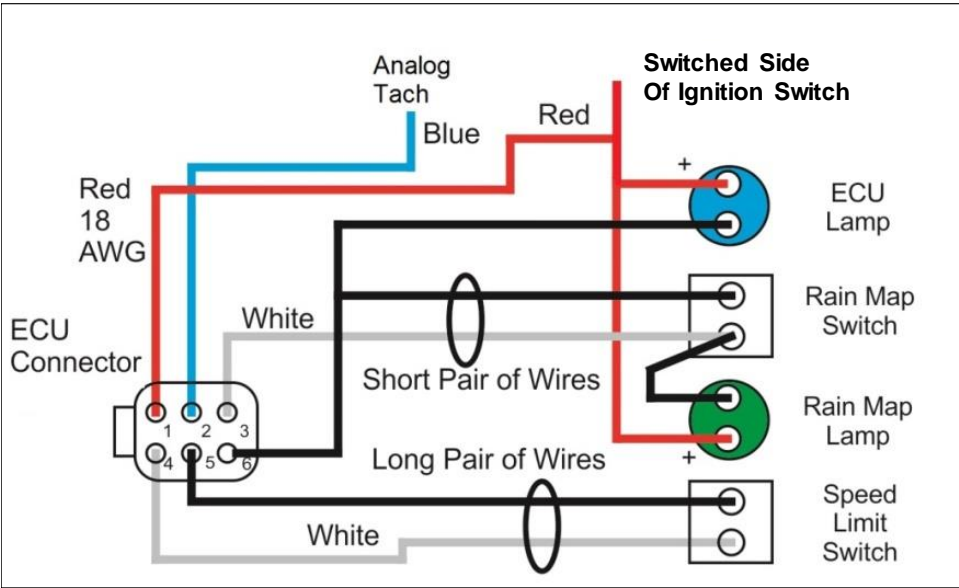
Figure A4 – G3 Dash Harness Schematic
