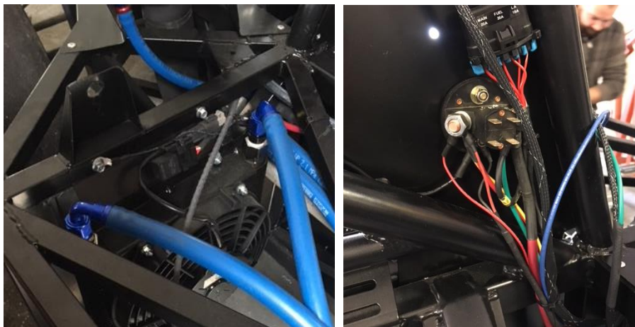
Figure 37 – Oil Cooler Harness (Pod & Engine View)
