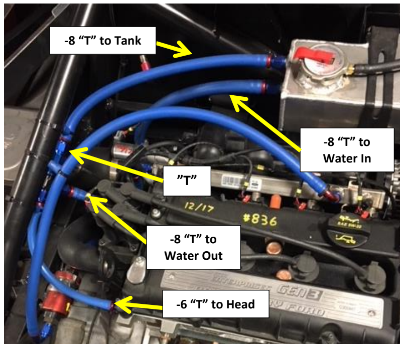
Figure 50 –Water Lines Connections
