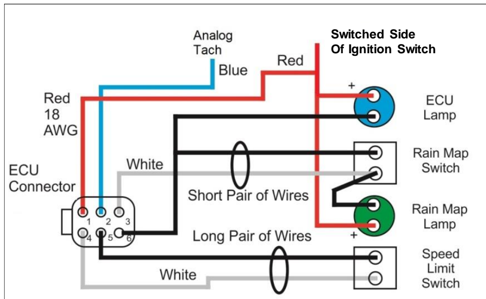
Figure 31 – Dash Wiring – ECU Connections/Side
