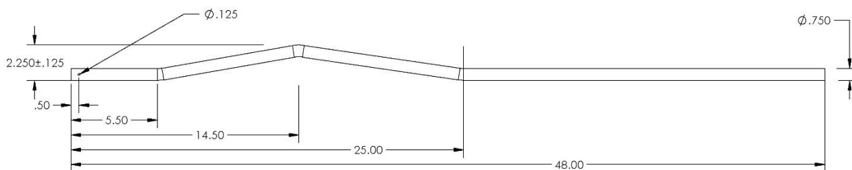
Figure 9 – Shift Shaft Modifications
