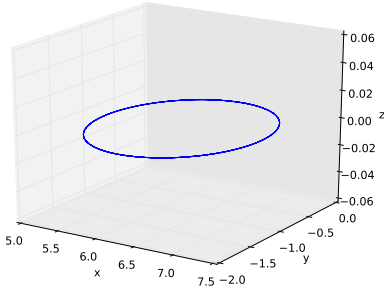
Figure 1: Uniform magnetic field in the z -plane. Initial velocity in x direction. Lorentz force acting in xy -plane making the particle move in a circle. Units are arbitrary.
