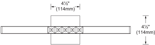
JB - Square canopy for 4" junction box Canopy to cover a standard 4" octagonal junction box.
