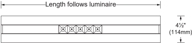
PB - Full length canopy for 4" junction box Long adapter plate to cover a standard 4" octagonal junction box.
