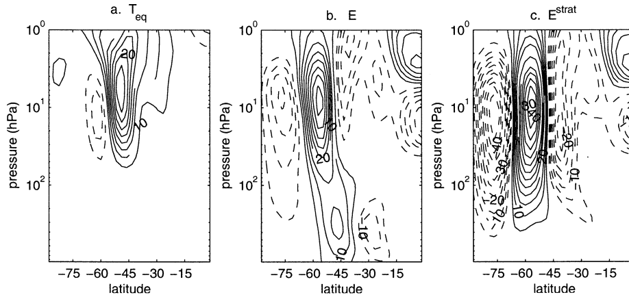
FIG. 7. (a) The quantity u[E(\gamma = 2), T_{eq}(\gamma = 4)] - u[E(\gamma = 2), T_{eq}(\gamma = 2)] described in the text, from the zonally symmetric model. The contour interval is 5 \text{ m s}^{-1} and the zero contour is not plotted. (b) As in (a) but for u[E(\gamma = 4), T_{eq}(\gamma = 2)] - u[E(\gamma = 2), T_{eq}(\gamma = 2)] . (c) As in (b) but for the eddy forcing perturbation confined to the stratosphere, E^{\text{strat}} [Eq. (11)].
