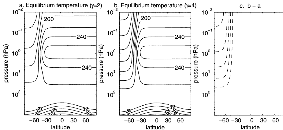
FIG. 1. (a) Plot of T_{eq} for \gamma = 2 \text{ K km}^{-1} . The contour interval is 20 K. (b) As in (a) but for \gamma = 4 \text{ K km}^{-1} . (c) The difference in T_{eq} between \gamma = 4 \text{ K km}^{-1} and \gamma = 2 \text{ K km}^{-1} , that is, (b) minus (a). The contour interval is 10 K, dashed contours denote negative values, and the zero contour is not plotted.
