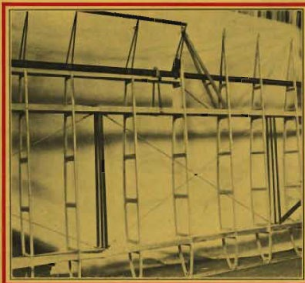
Structural section of Cardinal wing showing Tri-tube compression members, steel aileron and control tube.
