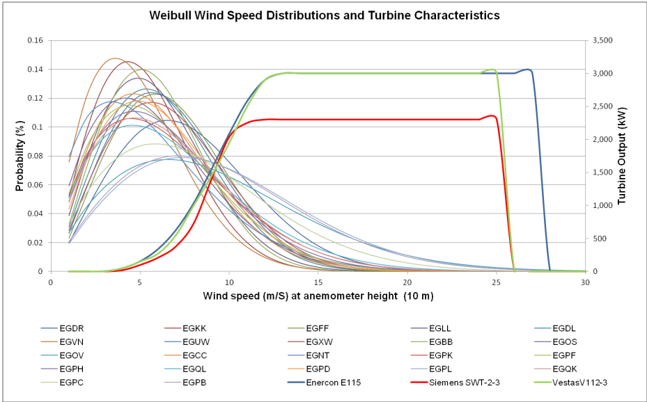
Figure 5 Wind probability functions and the turbine characteristics used in the model
