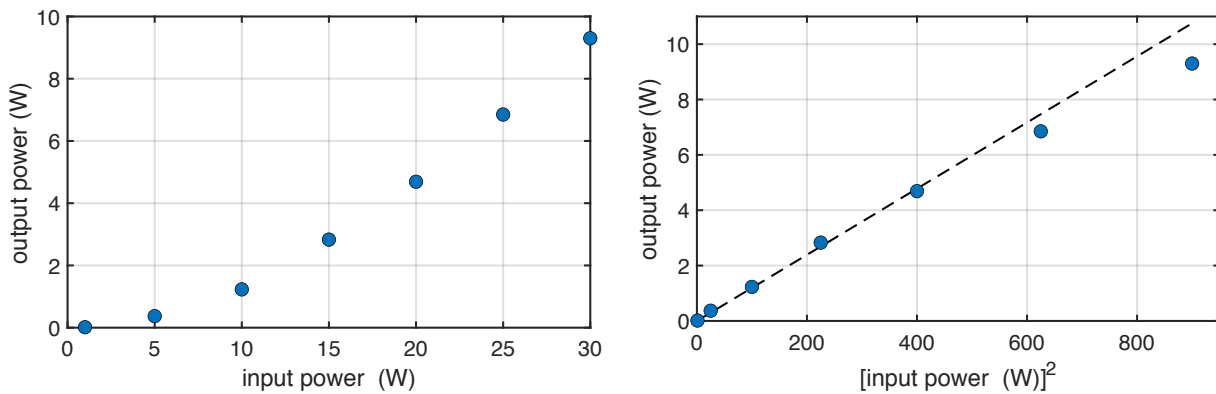
Figure 3.3: Frequency doubling efficiency. Variation of 532-nm output power versus 1064-nm (a) input power and (b) input power squared.
