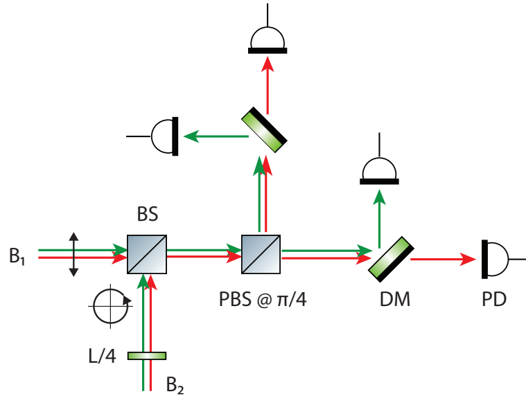
Figure 3.8: Optical part of the new scheme for generating phase lock error signals. Two low-power beams that are picked off from the lattice beams are directed into an interferometer. One of the two beams passes through a quarter waveplate and becomes circularly polarized. The two beams are then combined on a beam splitter. A polarizing beam splitter rotated by \pi/4 with respect to the optical table analyzes the combined light and separates it into two orthogonally polarized components. A dichroic mirror separates the two colors for each component. All the beams are detected by separate photodiodes. In the experiment, there are two copies of this setup for the two pairs of relative phases ( \theta_{12} and \theta_{23} ) for each color. Legend: L/4, quarter waveplate; BS, beam splitter, PBS: polarizing beam splitter; DM, dichroic mirror; PD, photodiode.
