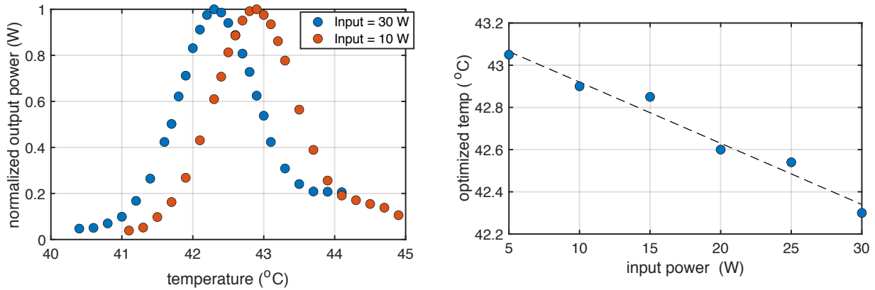
Figure 3.4: Temperature tuning of the frequency-doubling crystal. (a) Normalized output power of the doubling crystal at two different input powers (10 W and 30 W) measured with fixed beam alignment. (b) Optimized crystal temperature at different input powers.
