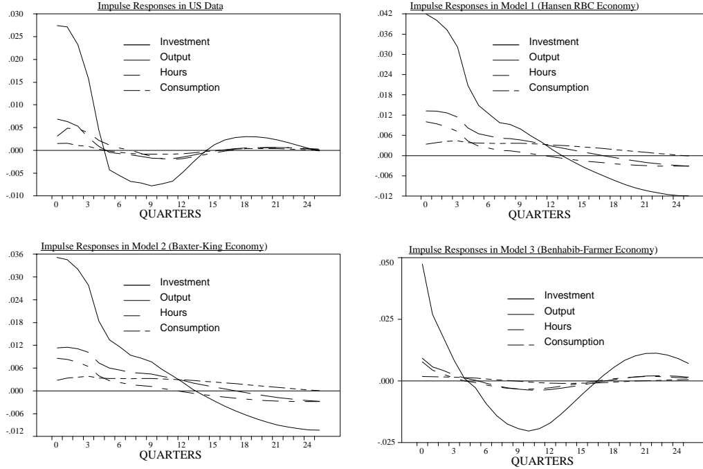
Figure 1: Three Simulated Impulse Responses Compared with US Data
