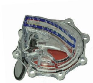
Above: FlowVis® retrofit model
