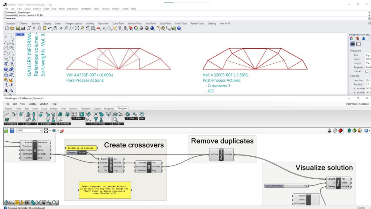
Figure 73 – An example of the output of the crossovers functionality
