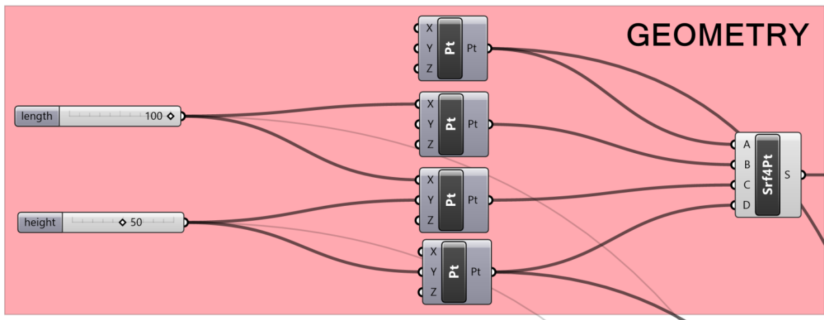
Figure 6 – Definition of the Design Domain within Grasshopper
