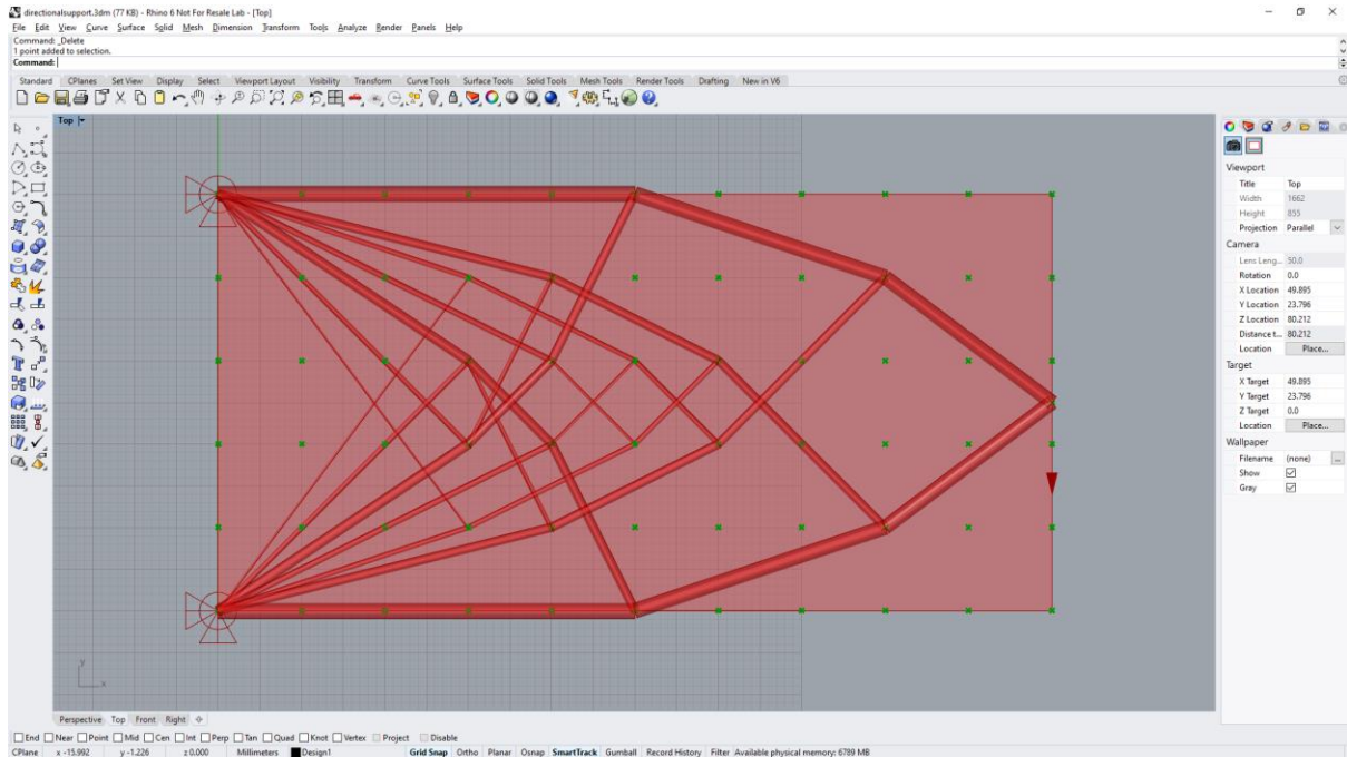
Figure 64 – The Simple2D problem in Rhino. Nodes previewed in green
