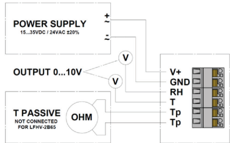
Fig. 2. Connection diagram, voltage output
