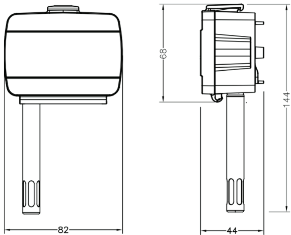
Fig. 1. Dimensions (mm / inch) 1/2" NPT conduit adapter & cable gland not shown
