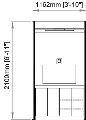
FRONT ELEVATION
