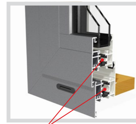
The 'thermal break' is made from polyimide which reduces the transference of cold or heat through the frame.
