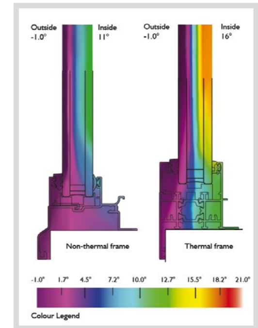
These thermal models show the same outside air temperature but a noticeable difference in the frame temperature on the inside.
