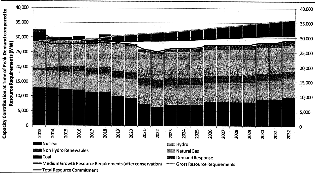
The graphic above reflects the Government's LTEP scenario indicating the need for new generation supply starting in 2019
