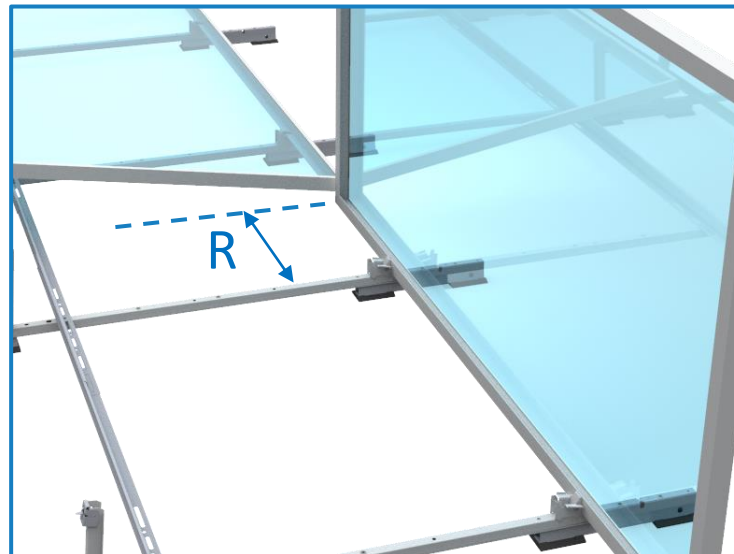
Tip: R dimension is found in the Racking Construction Set. See Sheet Title: Typical Array Dimensions.
