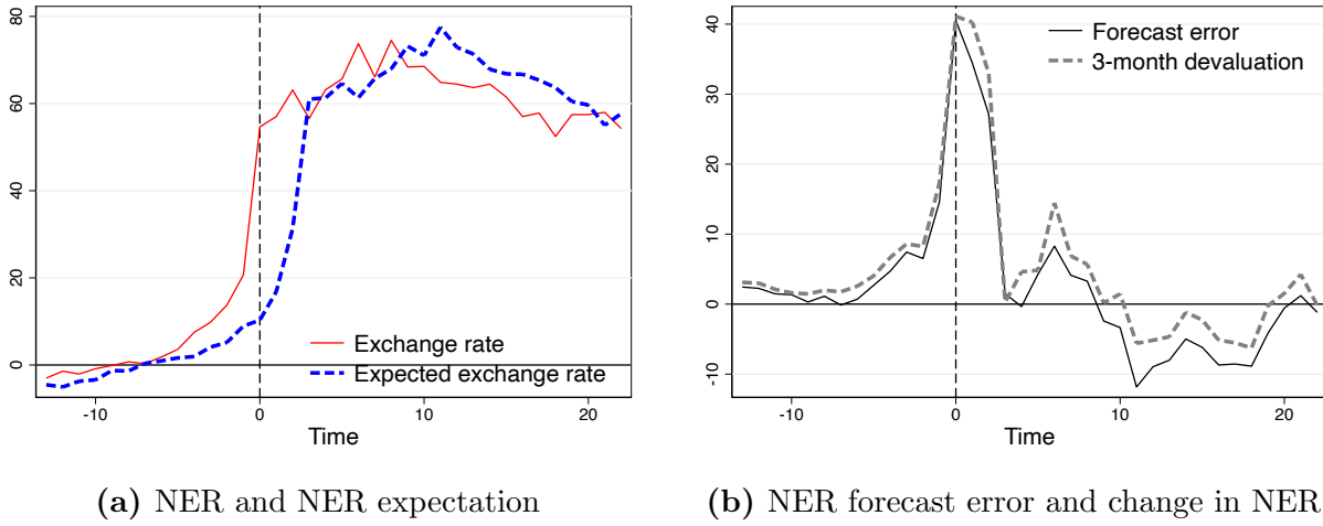
Figure B.12 – Predictability of the NER across Large Devaluation
