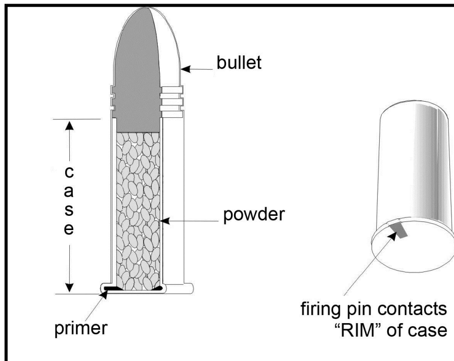
Figure 94. Rim-fire Cartridge
