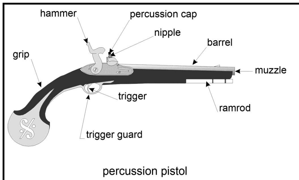
Figure 87. Muzzleloader
