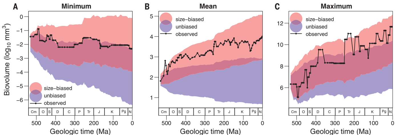
Fig. 2. Comparison of observed biovolume trends to those obtained from stochastic branching models (23). The colored regions highlight the size space occupied by 90% of the 1000 model runs. For clarity, only results for the size-biased (red) and unbiased (blue) models are shown; except below the minimum size, the lower-bounded model produced results nearly identical to the unbiased model (fig. S4). (A) Minimum, (B) mean, and (C) maximum sizes. Time scale abbreviations are the same as in Fig. 1.
