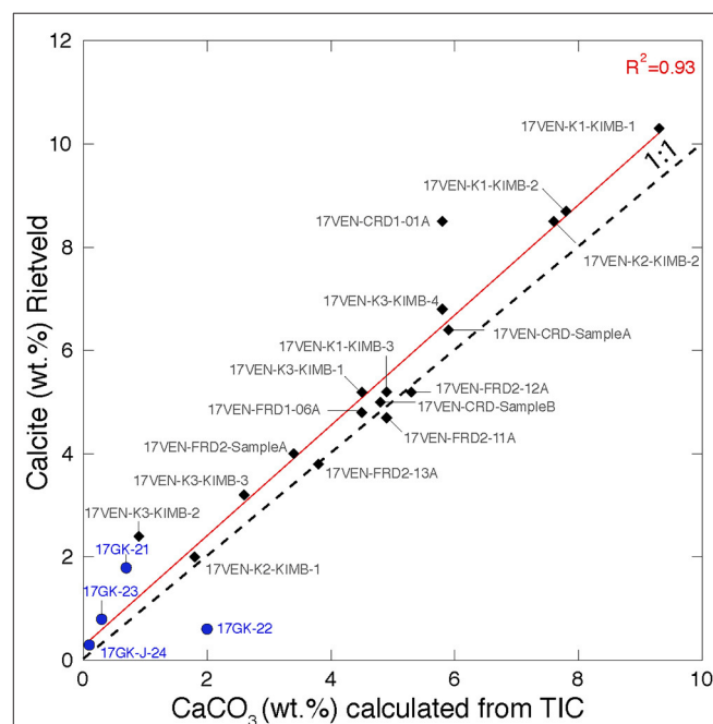
FIGURE 3 | Biplot representing \text{CaCO}_3 abundances calculated from bulk TIC analyses (measured by coulometry) vs. the calcite content (wt.%) determined by Rietveld refinement. The R^2 of the regression line is 0.93 and close to the 1:1 line supporting the accuracy of the calcite estimation using Rietveld refinement. Samples from Venetia are represented by black diamonds and samples from Gahcho Kué are represented by blue circles. Samples from the Gahcho Kué mine are calcite and TIC-poor.
