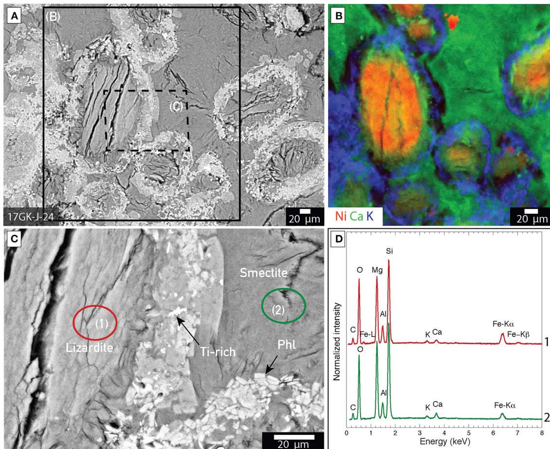
FIGURE 6 | Distribution of mineral phases within kimberlite ores from Gahcho Kué (17GK-J-24). (A) Backscattered electron image of a petrographic thick section showing lizardite grains (after forsterite) surrounded by bright rims and a smectite matrix; (B) XFM map of Ni (red), Ca (green) and K (blue) of the area marked by a solid rectangle in (A) . The red, green and blue colors correspond to the measured intensities of the Ni K-alpha, Ca K-alpha and K K-alpha emission lines, with the brightest color, the highest measured count rate and black corresponding to the lowest count rate; (C) Close up corresponding to the dashed rectangle in (A) showing that the rim is composed of talc, Ti-rich grains (Ti), likely ilmenite, and phlogopite (Phl); (D) SEM-EDXS spectrum of the circled area in (B) .
