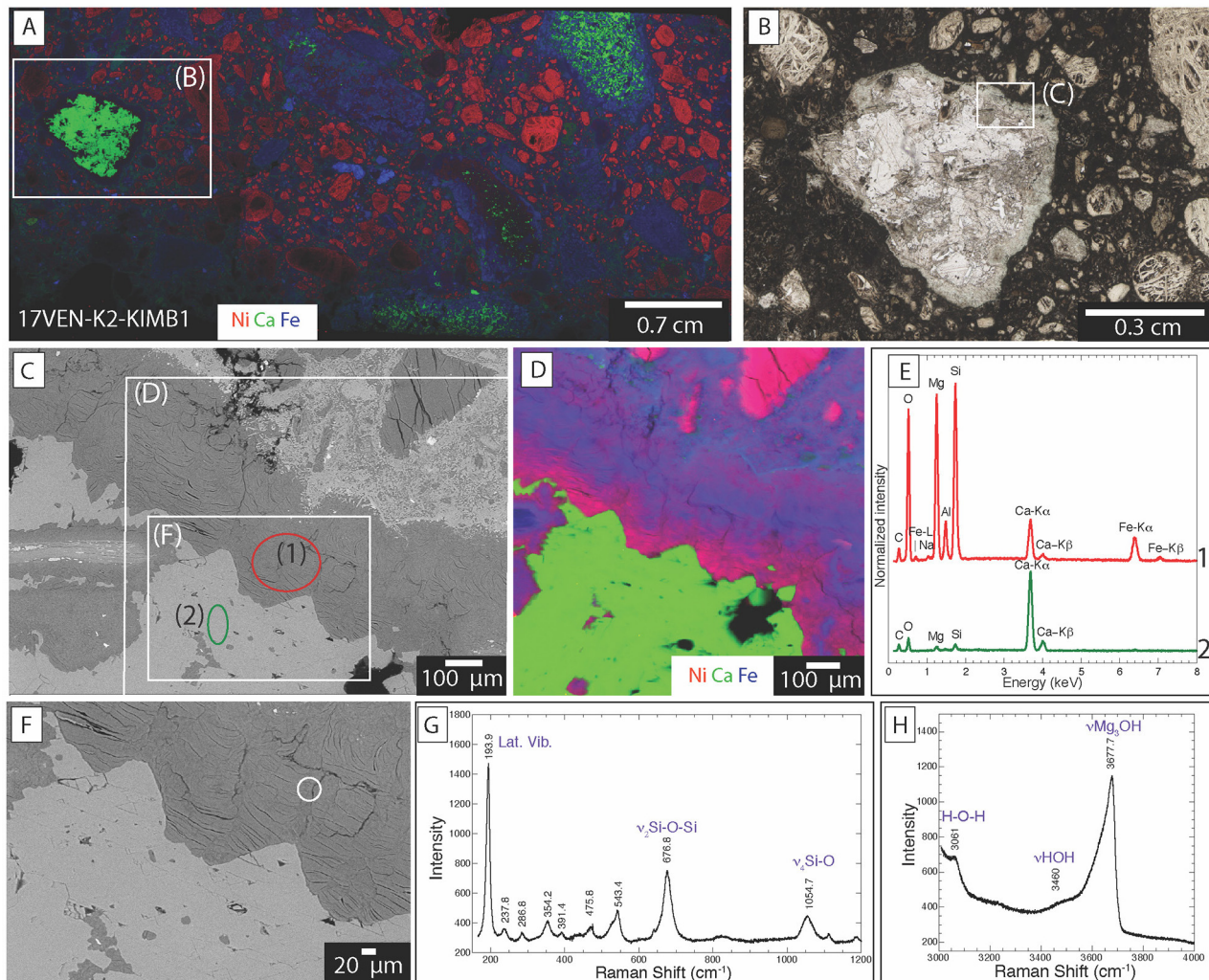
FIGURE 7 | Distribution of mineral phases within kimberlite ores from Venetia (17VEN-K2-KIMB1) (A) XFM map showing the distribution of Ni (red), Ca (green) and Fe (blue) of the entire thin section. The red, green and blue colors correspond to the measured intensities of the Ni K-alpha, Ca K-alpha and Fe K-alpha emission lines, with the brightest color, the highest measured count rate and black corresponding to the lowest count rate; (B) Optical photograph of the area marked by a rectangle on (A) showing agglomeration of calcite crystals; (C) Backscattered electron image of the area marked by a rectangle in (B) at the interface between the matrix and the polycrystalline calcite grain; (D) XFM map showing the distribution of Ni, Ca and Fe. The red, green and blue colors correspond to the measured intensities of the Ni K-alpha, Ca K-alpha and Fe K-alpha emission lines, with the brightest color, the highest measured count rate and black corresponding to the lowest count rate. (E) Backscattered image of the area marked on (C) ; (G,H) Raman spectra of the areas circled in (F) .
