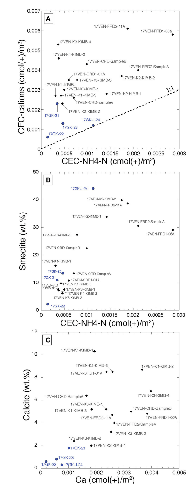
FIGURE 4 | Biplots representing (A) the CEC determined by the \text{NH}_4\text{-N} concentrations in the KCl leachates (CEC- \text{NH}_4\text{-N} ) vs. the CEC determined by the sum of the cations measured in the first \text{NH}_4\text{-acetate} leachates (both BET (Continued)
