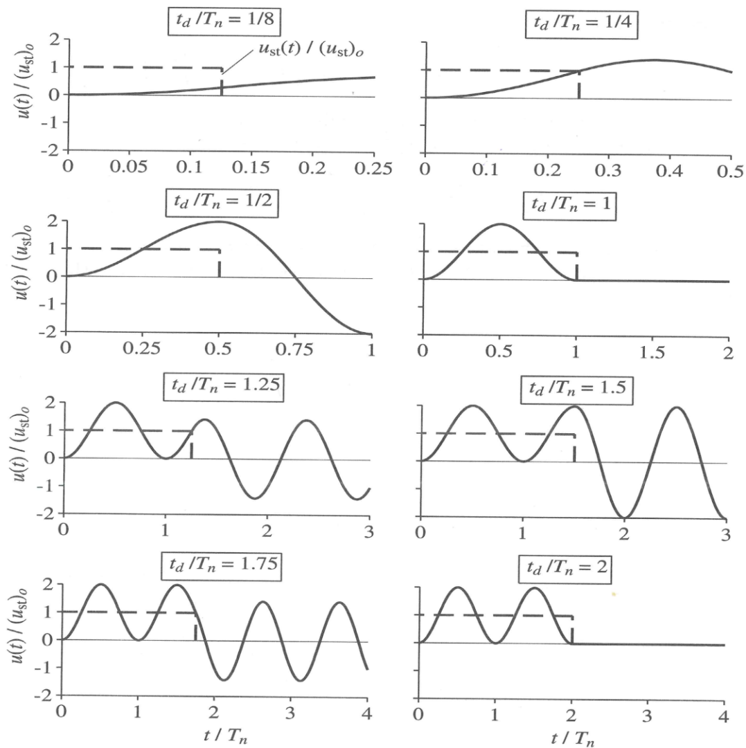
Dynamic response of undamped SDF system to rectangular pulse force; static solution is shown by dashed lines.
