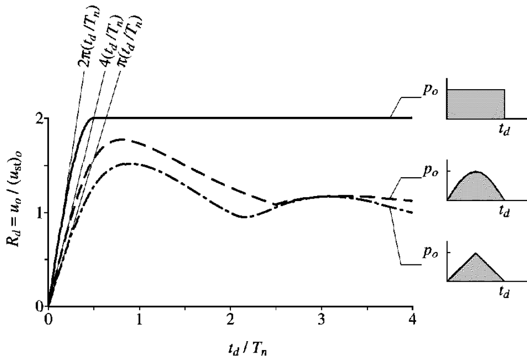
Shock spectra for three force pulses of equal amplitude.
