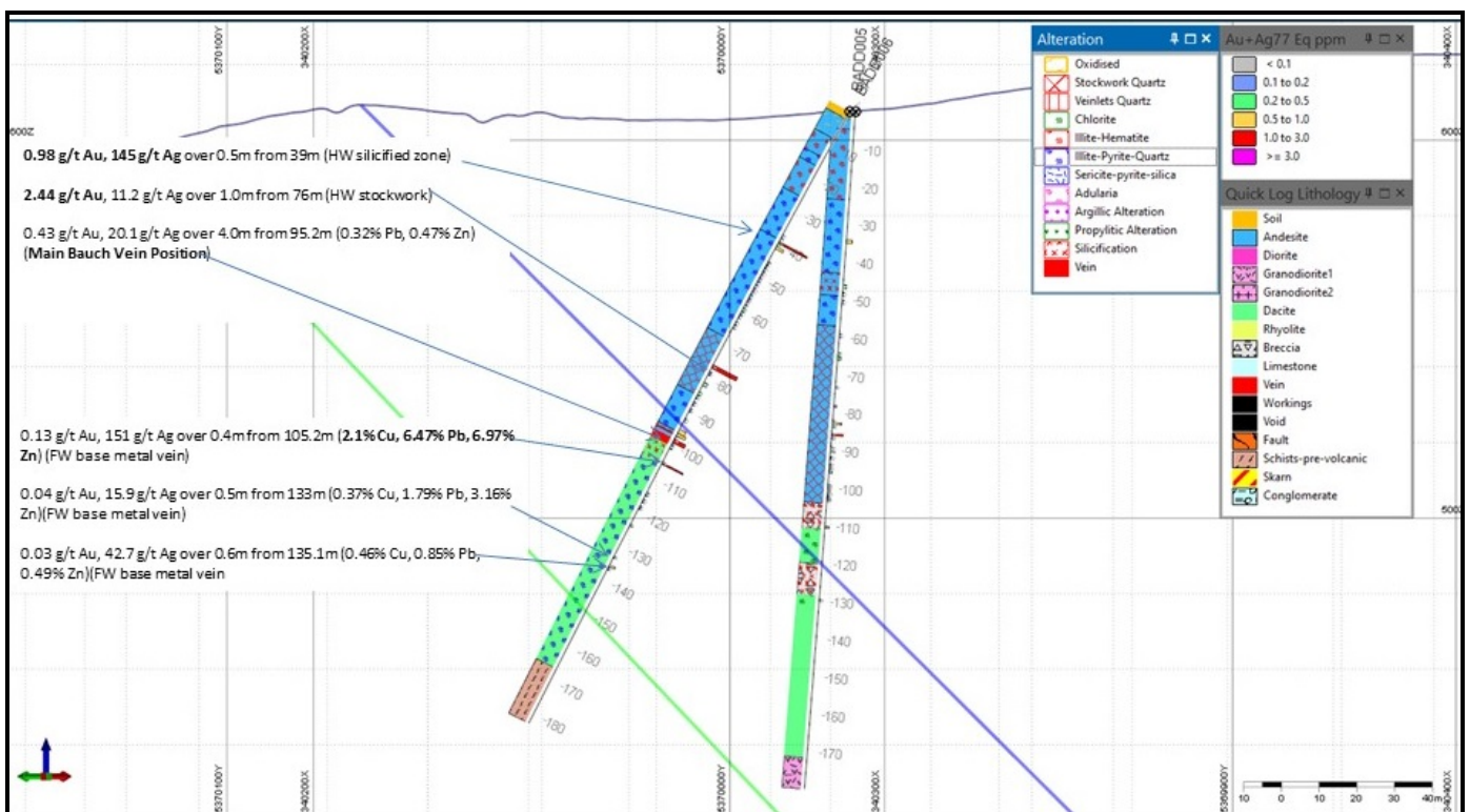
Cross section through the LNF structure. BADD006 visible gold occurred at 76.0m in a hanging wall stockwork within the LNF.
