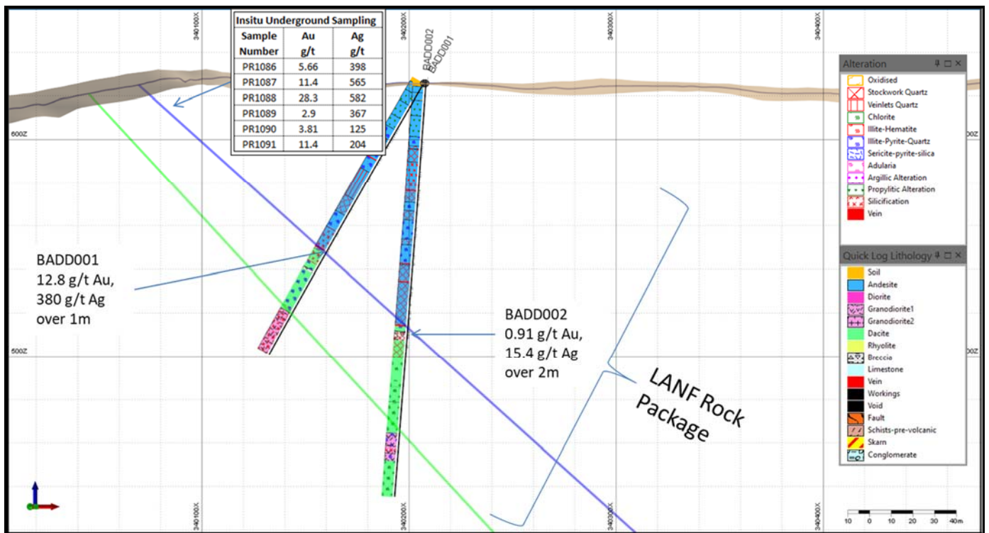
Cross section through the LNF structure. BADD001 gold and silver mineralisation occurs in the Bauch vein position which is open up and down dip and along strike. The footwall granodiorite contact also has potential to host gold, silver and/or base metal mineralised shoots.
