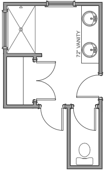
MASTER BATH OPTION "A"
