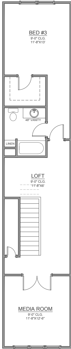
RIVERSIDE UPPER FLOOR PLAN
