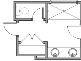
MASTER BATH OPTION "A"
