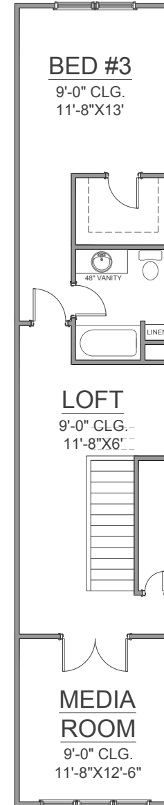
RIVERSIDE UPPER FLOOR PLAN
