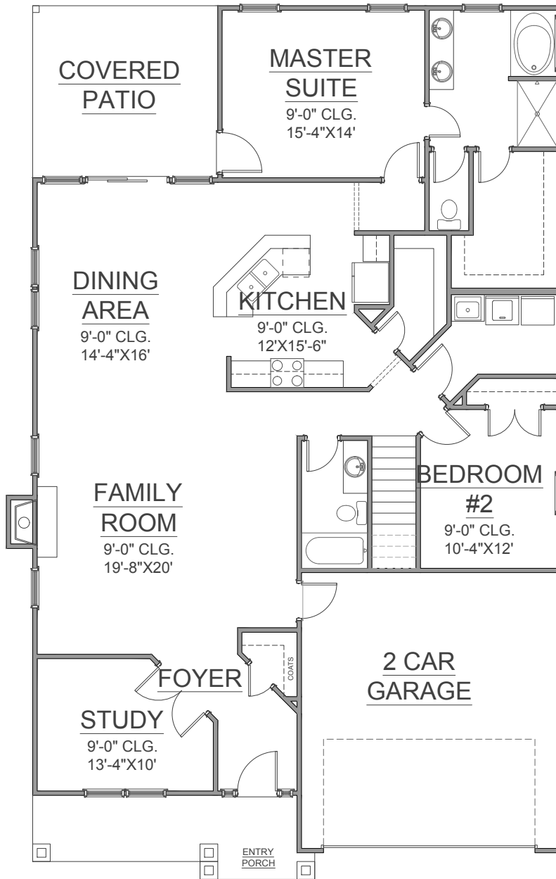
RIVERSIDE MAIN FLOOR PLAN
