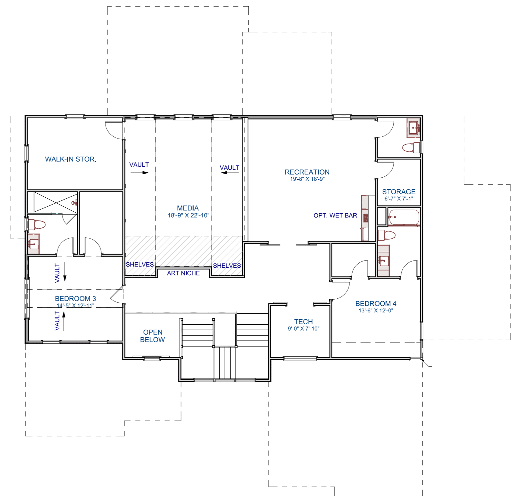
Second Floor
