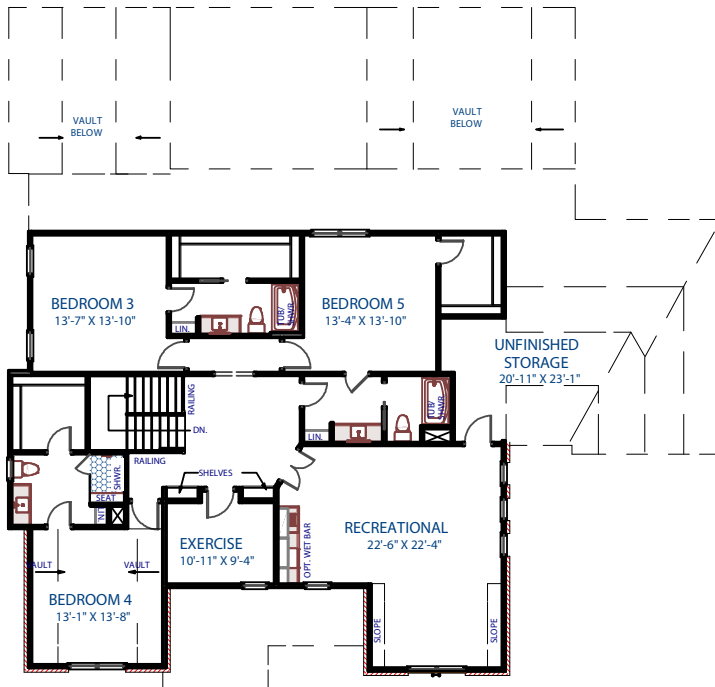
Second Floor
