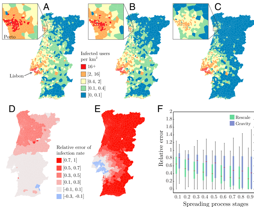
Fig. 5. Epidemic spreading simulations in Portugal. Densities of infected users at time t = 17 following a simulation of an SIS spreading process ( \mu = 0.9, \nu = 0.3 ) originated from Lisbon by using (A) real mobility fluxes T^M , (B) the rescaled social fluxes \tilde{T}^S , and (C) the mobility fluxes approximated by gravity model T_{GM}^M . (D) Relative errors of infection rate \bar{e}_r(t) (Eq. S19) and (E) \bar{e}_r^{gm}(t) (Eq. S20) at each location i at time t = 17 . (F) Distributions of mean relative error \bar{e}(t) (green) and \bar{e}^{gm}(t) (blue) over 500 SIS simulations at different stages before reaching the steady state, documenting the superior predictive power of our method comparing with gravity model at all stages of the spreading processes.
