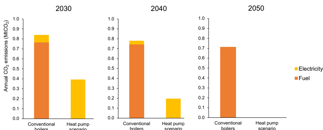
Figure 20. Annual CO 2 emissions for steam generation from textile wet-processing industry in Taiwan (technical potential assuming a 100% adoption of industrial heat pump applications).
