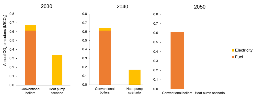
Figure 19. Annual CO 2 emissions for steam generation from textile wet-processing industry in Japan (technical potential assuming a 100% adoption of industrial heat pump applications).
