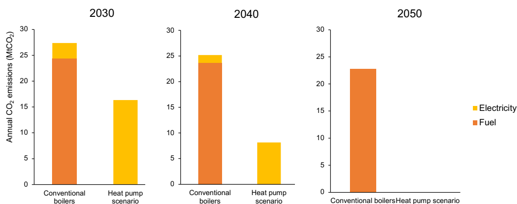
Figure 18. Annual CO 2 emissions for steam generation from textile wet-processing industry in China (technical potential assuming a 100% adoption of industrial heat pump applications).
