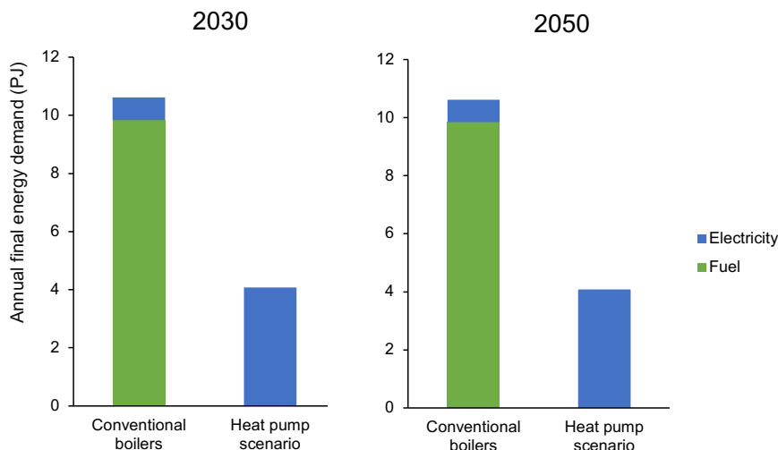
Figure 17. Annual final energy demand for steam generation in the textile wet-processing industry in Taiwan (technical potential assuming a 100% adoption of industrial heat pump applications).
