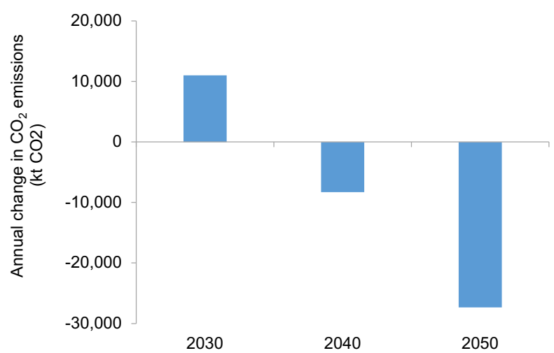
Figure 25. Potential change in steam boilers’ annual CO 2 emissions after electrification in the textile industry in China (technical potential assuming a 100% adoption rate).
