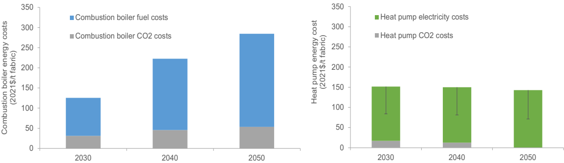
Figure 21. Energy costs per unit of production for steam generation in the textile wet-processing industry in China .
