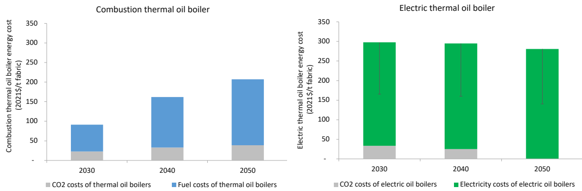
Figure 35. Energy costs per unit of production for combustion and electric thermal oil boilers in the textile wet-processing industry in China .
