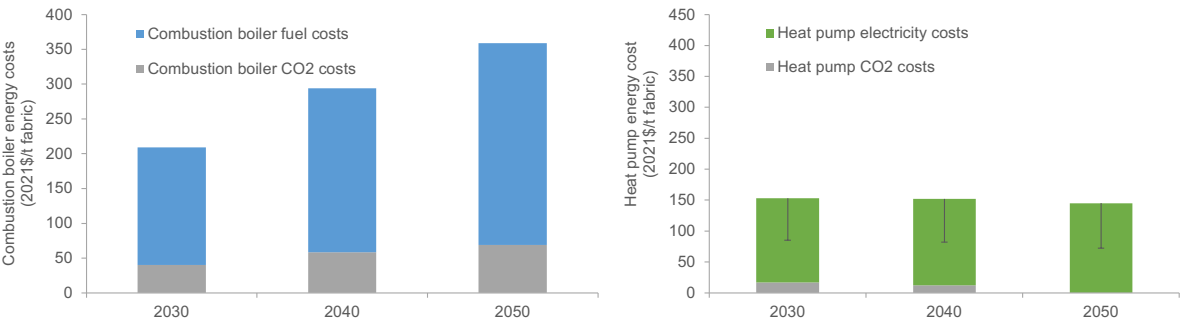
Figure 23. Energy costs per unit of production for steam generation in the textile wet-processing industry in Taiwan .
