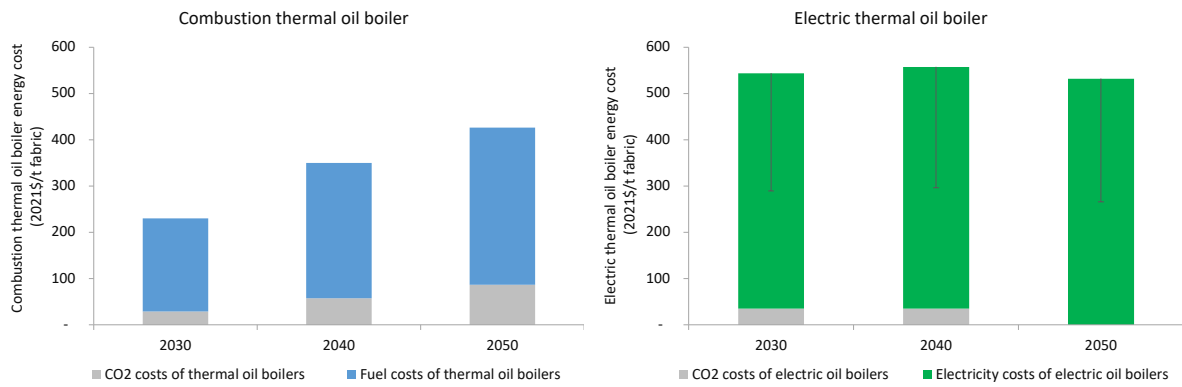
Figure 36. Energy costs per unit of production for combustion and electric thermal oil boilers in the textile wet-processing industry in Japan .
