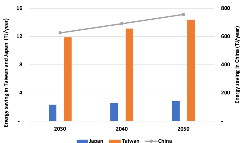
Figure 68. Total annual energy saving after electrification of yarn dyeing process (This is the technical potential assuming 100% adoption rate.)
