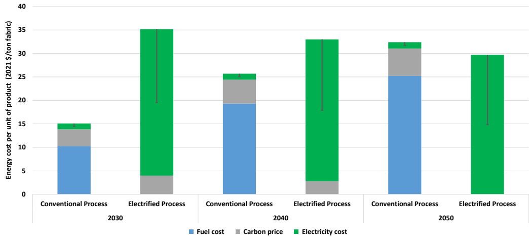
Figure 45. Energy cost per unit of production for conventional and electrified mercerizing and washing processes in China . (Note: The error bars show the energy cost per unit of production when the unit price of electricity is reduced by 50 %.)
