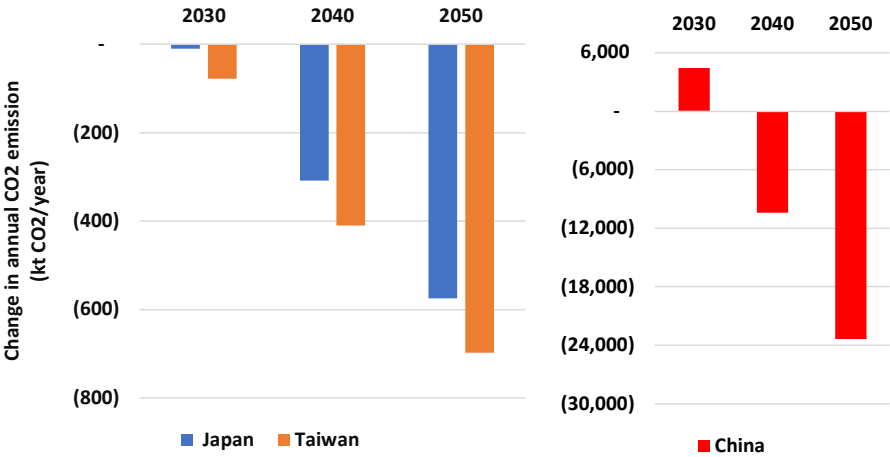
Figure 74. Total combined change in annual CO 2 emission after electrification of all seven studied wet-processing processes (This is technical potential assuming a 100% adoption rate.)
