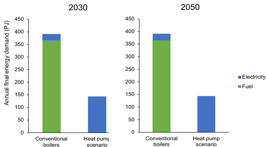
Figure 15. Annual final energy demand for steam generation in the textile wet-processing industry in China (technical potential assuming a 100% adoption of industrial heat pump applications).
