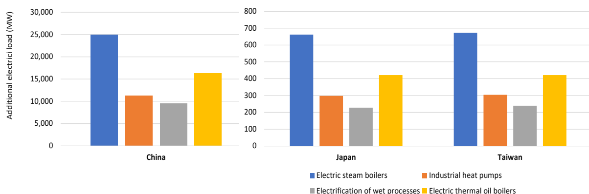
Figure 77. The total increase in electrical load (MW) after electrification under each technology pathways (This is the technical potential assuming a 100% adoption rate.)
