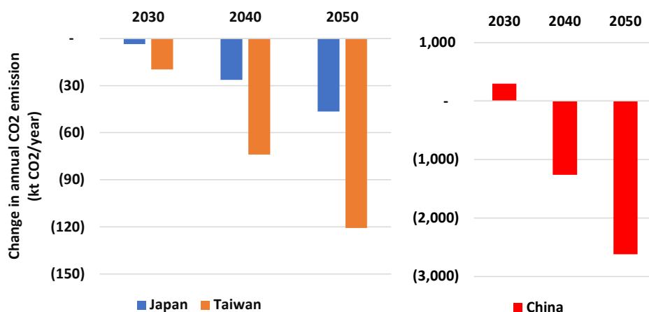
Figure 39. Total change in annual CO 2 emissions after electrification of singeing process (This is the technical potential assuming 100% adoption rate.)
