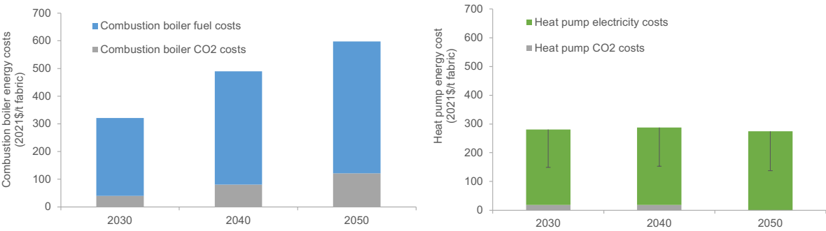
Figure 22. Energy costs per unit of production for steam generation in the textile wet-processing industry in Japan .
