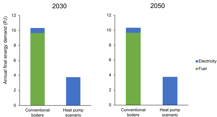
Figure 16. Annual final energy demand for steam generation in the textile wet-processing industry in Japan (technical potential assuming a 100% adoption of industrial heat pump applications).
