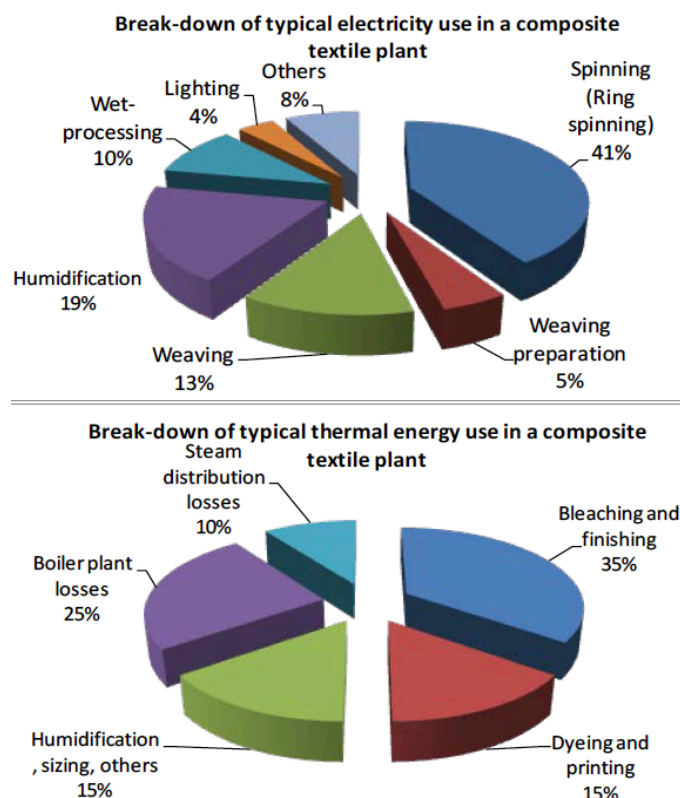
Figure 9. Breakdown of typical electricity and thermal energy used in a composite textile plant (Hasanbeigi 2010).
