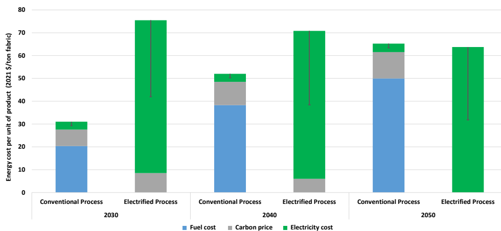
Figure 55. Energy cost per unit of production for conventional and electrified drying processes in China (Note: The error bars show the energy cost per unit of production when the unit price of electricity is reduced by 50 %.)
