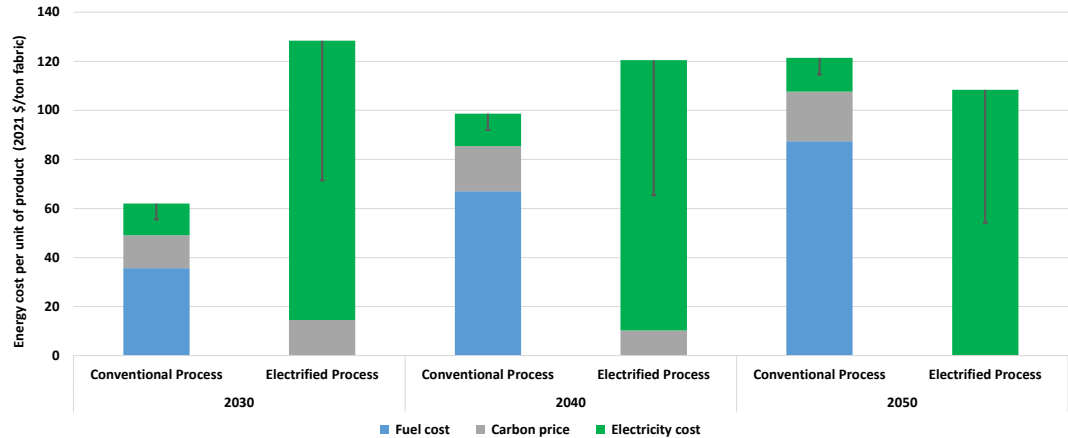
Figure 50. Energy cost per unit of production for conventional and electrified dyeing processes in China (Note: The error bars show the energy cost per unit of production when the unit price of electricity is reduced by 50 %.)
