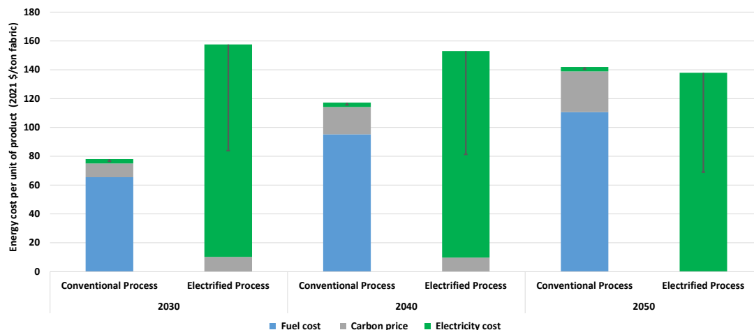
Figure 61. Energy cost per unit of production for conventional and electrified heat setting process in Japan .
