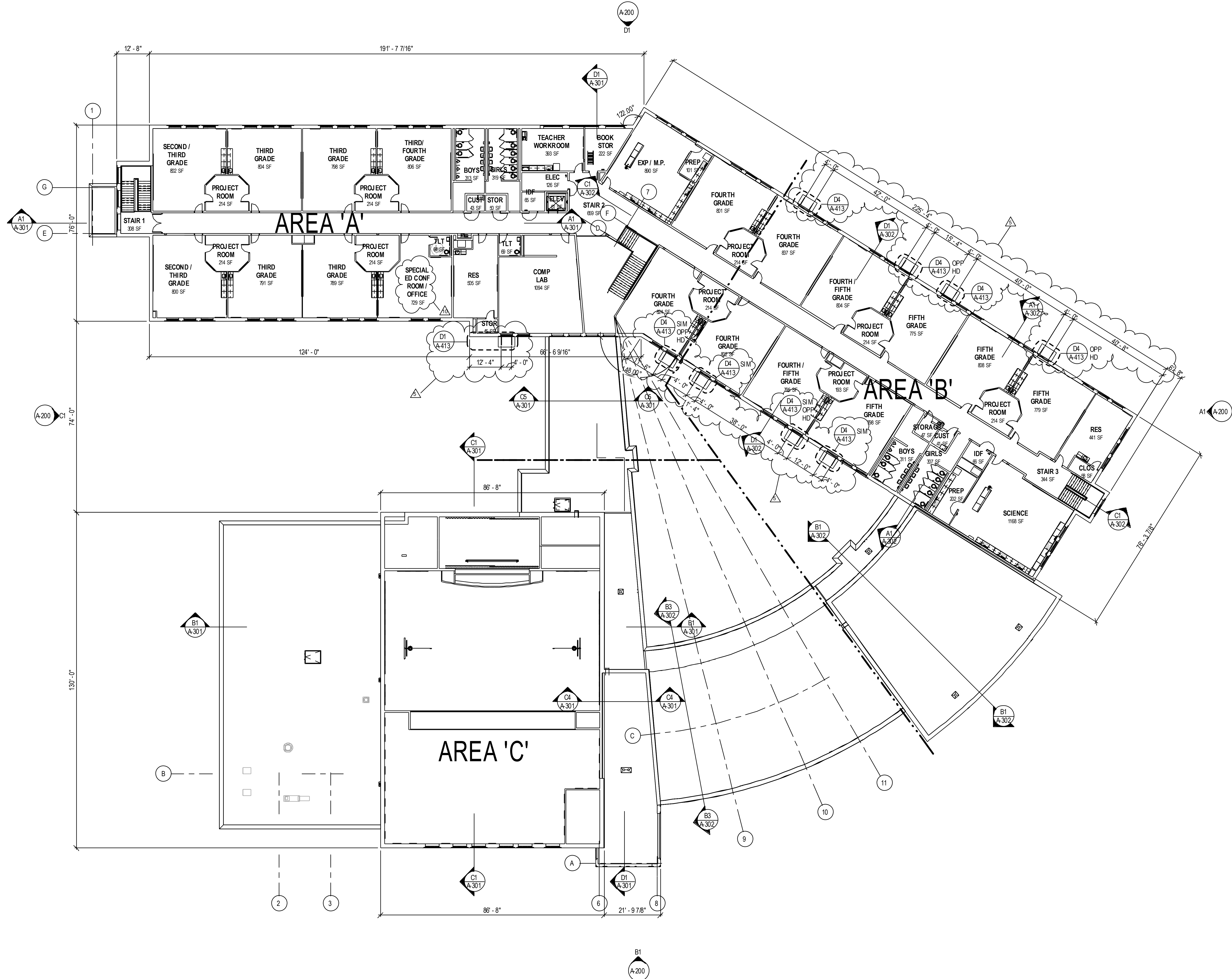
OVERALL SECOND FLOOR PLAN SCALE: 1/16" = 1'-0" PLAN NORTH
