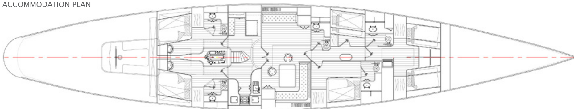
ACCOMMODATION PLAN
