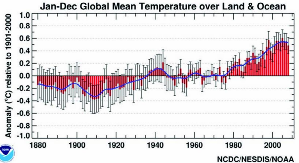
Graph B. Amount by degrees C that average annual global temperatures were above or below the 100-year average.
