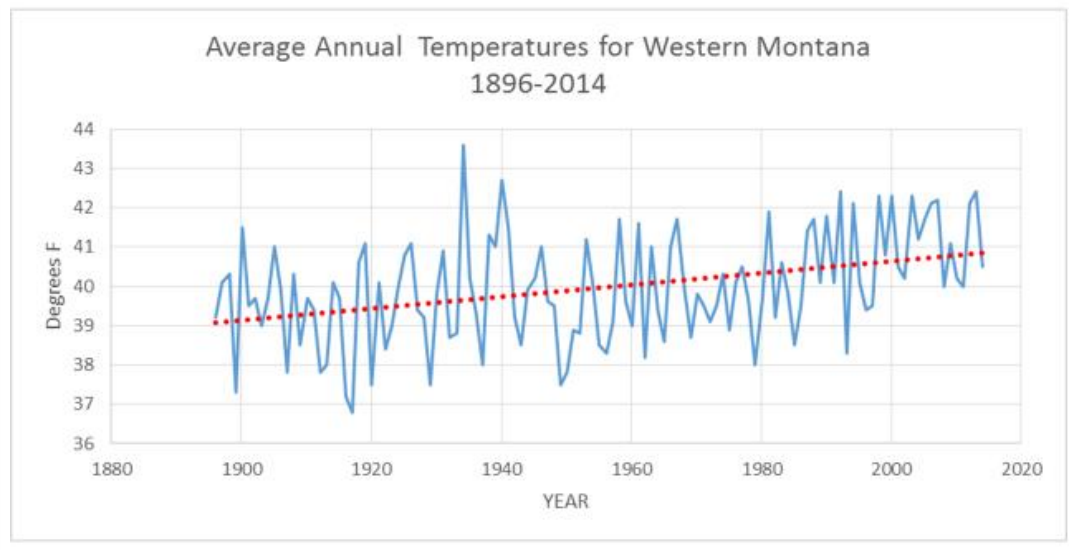
Graph D. Air temperature averaged across western Montana for each year since 1896 (blue line) and the trend in temperatures from 1896-2014 (red line).
