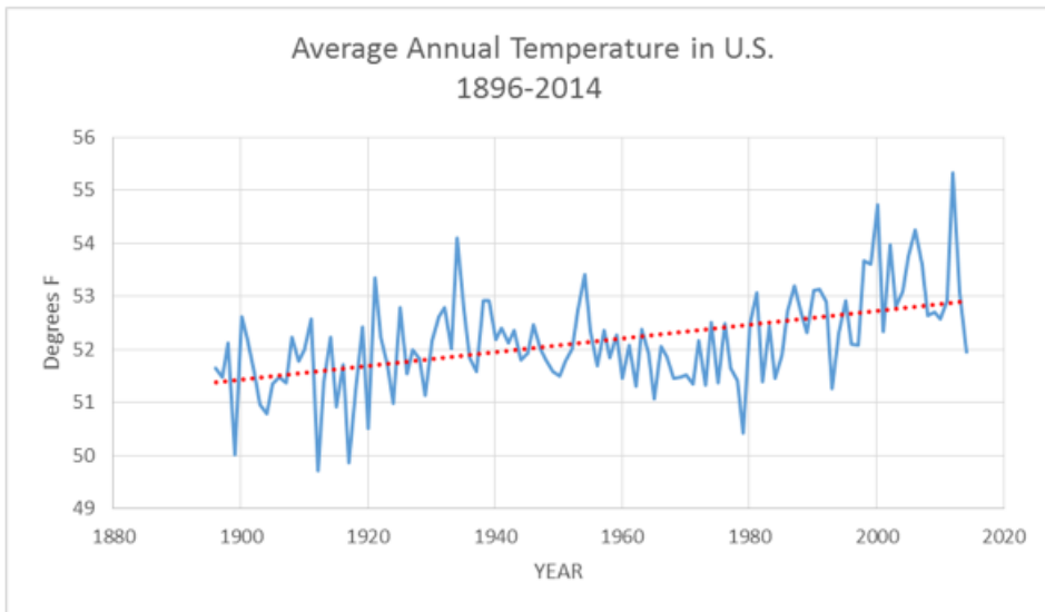
Graph C. Air temperature averaged across the contiguous United States for each year since 1896 (blue line) and the trend in temperatures from 1896-2014 (red line).
