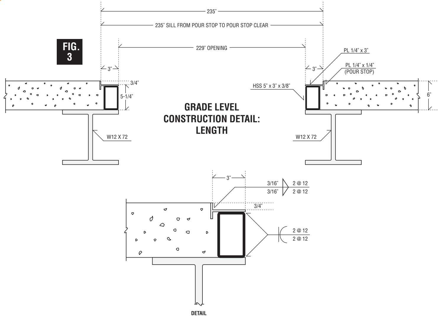
EDGE DETAIL SAMPLE USING TUBE STEEL OVER STRUCTURAL BEAM
