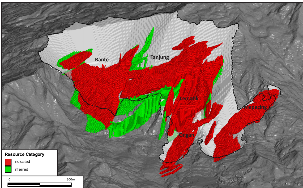
Figure 1: Awak Mas Deposit (isometric view looking south) showing Mineral Resource using May 2018 Mineral Resource shell
