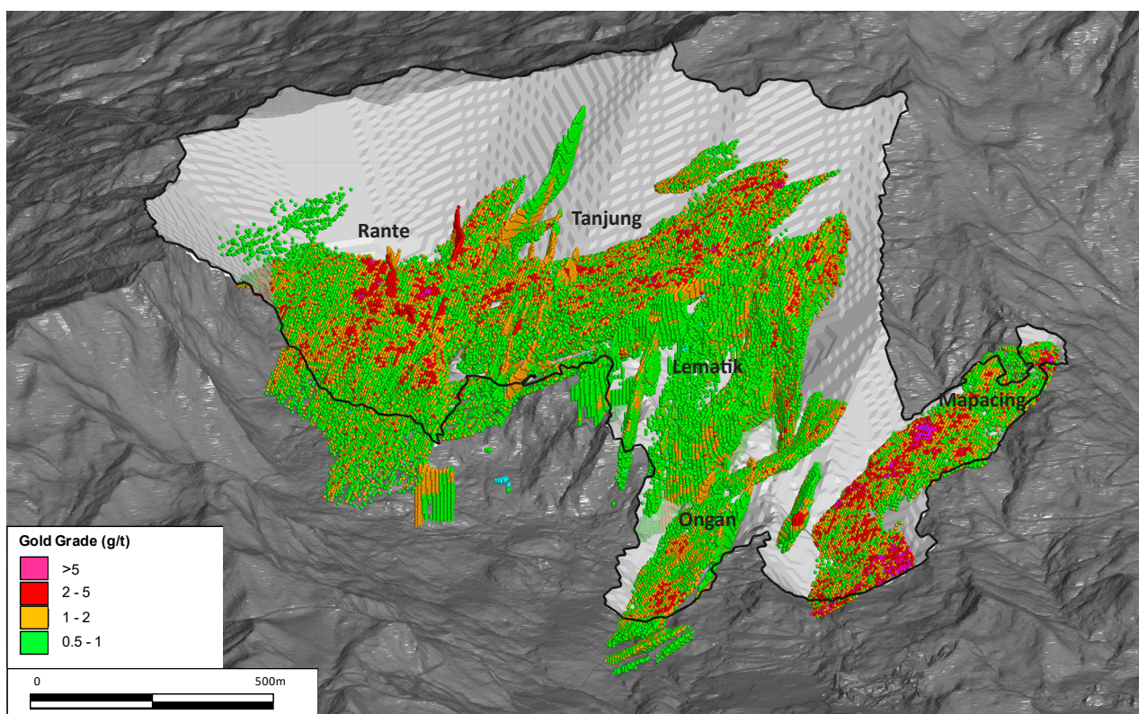
Figure 2: Awak Mas Deposit (isometric view looking south) showing Mineral Resource grades > 0.5 g/t Au using May 2018 Mineral Resource shell
