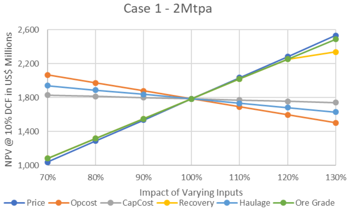
Figure 1 Scoping Study Update: Single parameter sensitivity analysis for the NPV - Case 1 (2Mtpa) (accurate to ±35% and includes US$36M contingency)
