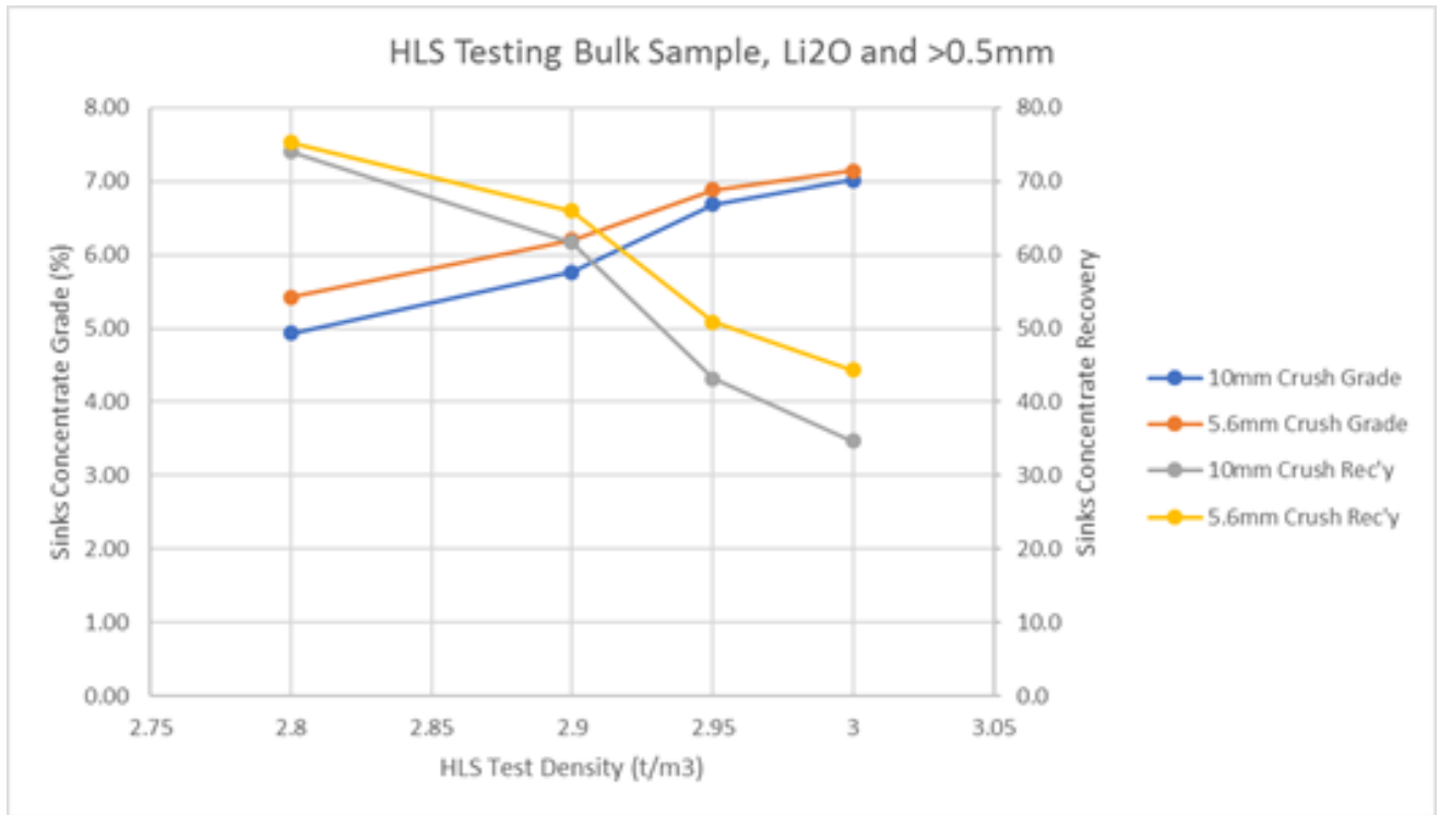
Figure 2. HLS Test work on Roche Dure Bulk Sample
