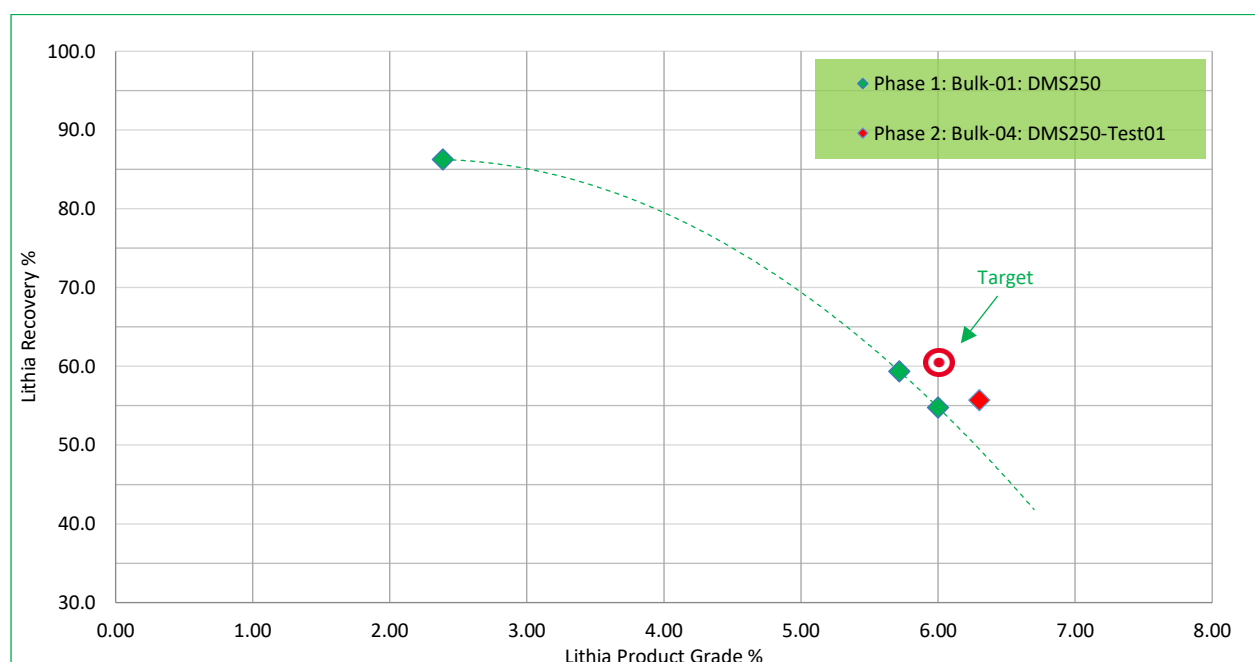
Figure 1 - Phase 2 Metallurgical Testwork 250 mm Preliminary Dense Media Cyclone Performance Curve
