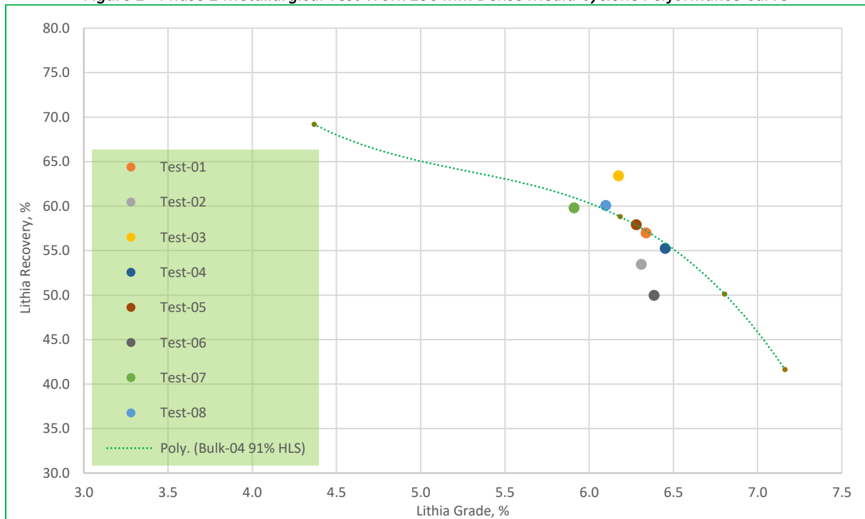
Figure 1 - Phase 2 Metallurgical Test Work 250 mm Dense Media Cyclone Performance Curve
