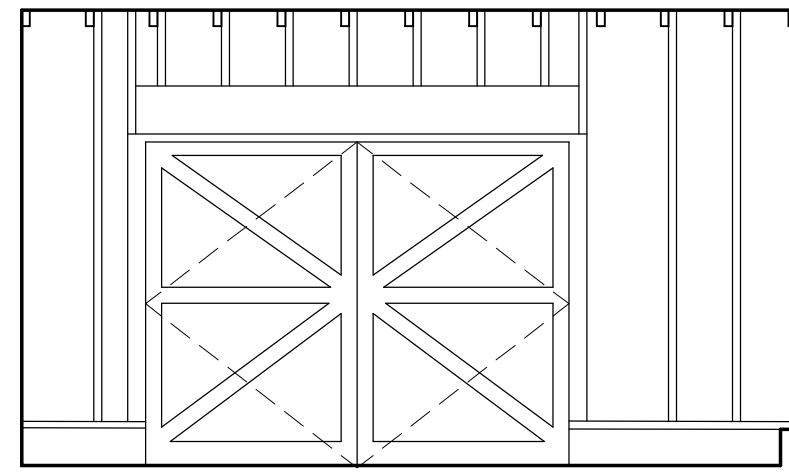
SHED/GALLERY Elevation 1
