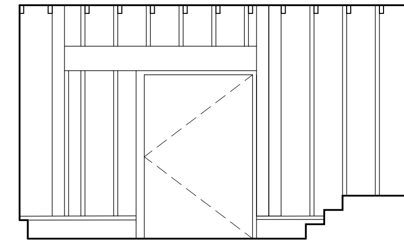
SHED/GALLERY Elevation 3
