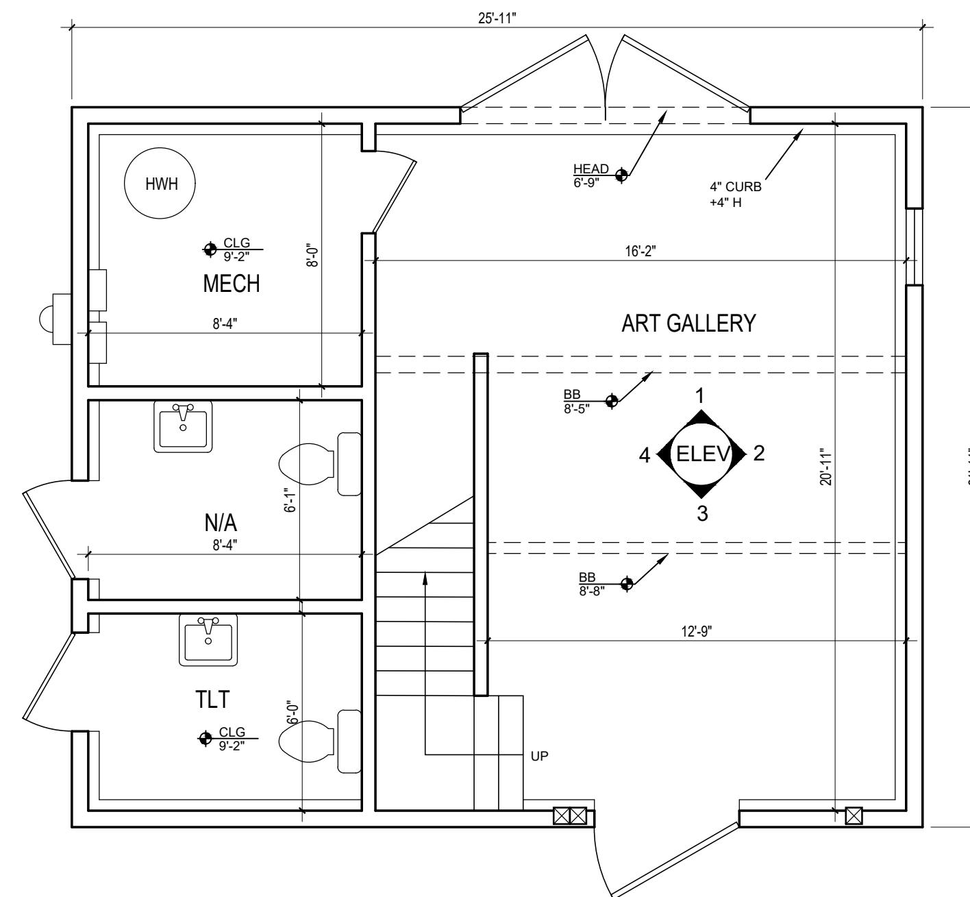
SHED/GALLERY 1st FI Plan
